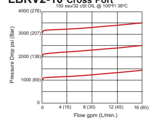
LBRV2-10 Cross Port
