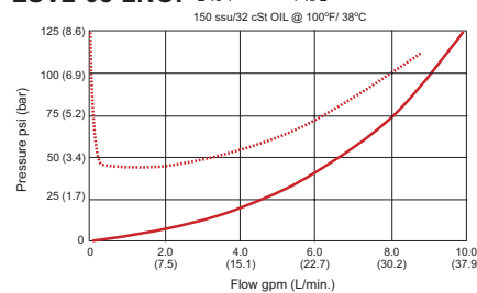
LSV2-08-2NOP 2 To 1 — 1 To 2 .....
