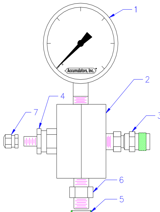
6000 psi Permanent Mount Pressure Monitor AI-PM6-000-SS
