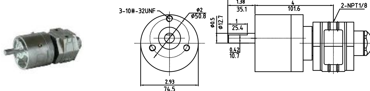
FS-4AM-RV-10 (Face or Foot mounting)
