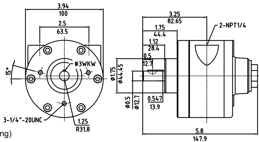
FS-4AM-V (Face mounting)
