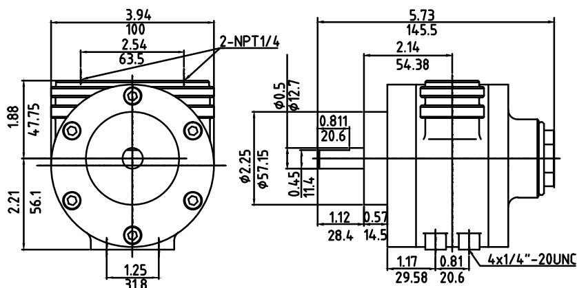
FS-NL32 (Hub &amp; Foot mounting)
