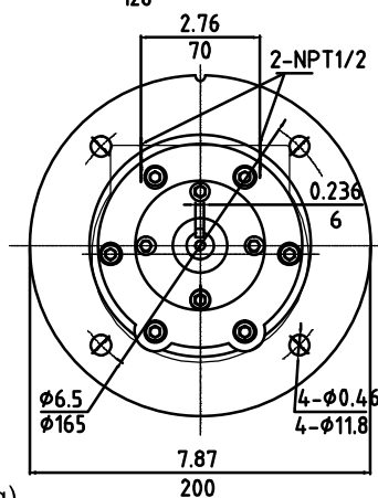
FS-6AM-F130 (IEC flange mounting)
