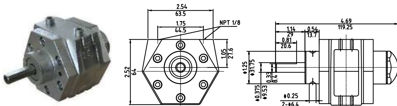
FS- 1UP-NRV (Hub mounting) (Reversible)
