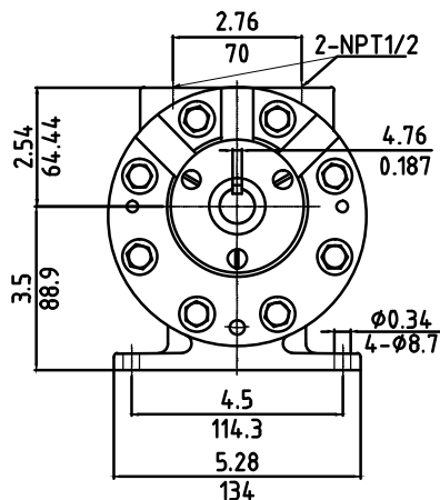
FS-8AM-H (Foot mounting)
