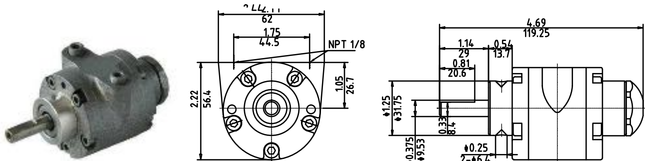
FS- 1UP-NCW (Hub mounting) (CW Rotation)
