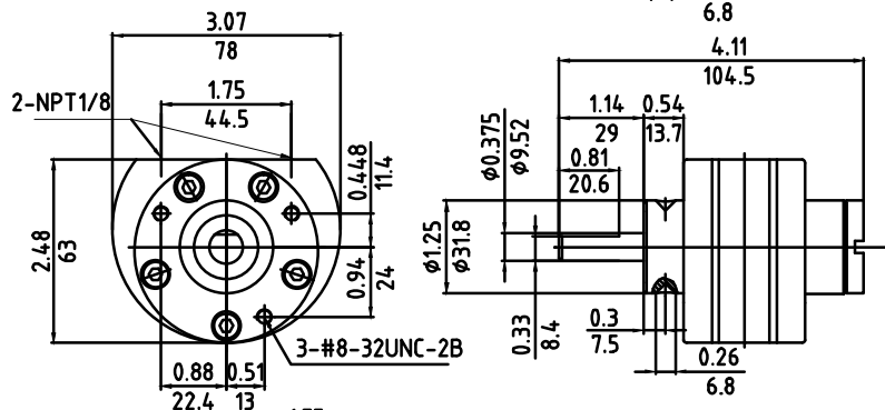
FS-1AM-VF-S-113 (Face mounting)
