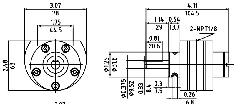
FS-1AM-V-S-113 (Hub mounting)
