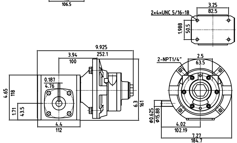
FS-WG02 (Base mounting)
