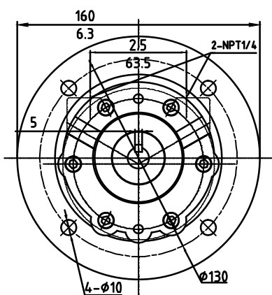
FS- 2AM-F110 (IEC flange mounting)
